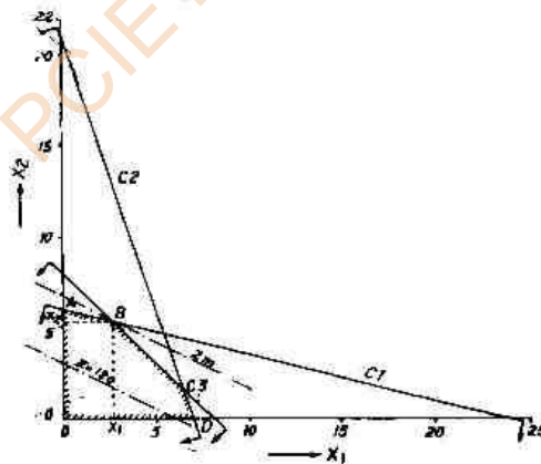
Fig. 11.2. Graphical method.
